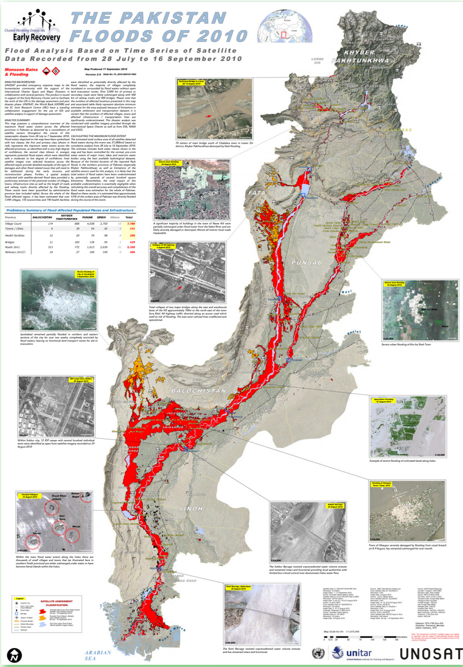
Flood analysis in Pakistan based on time series of satellite data recorded from 28 July to 16 September 2010. Credits: © UNOSAT.
